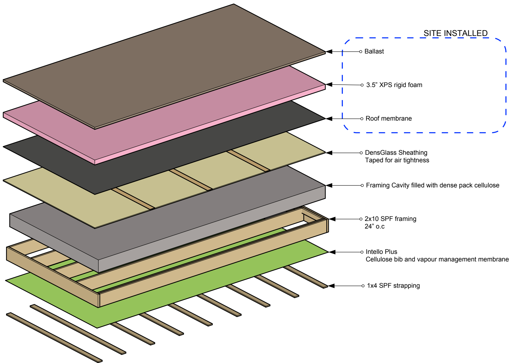
Exploded View
